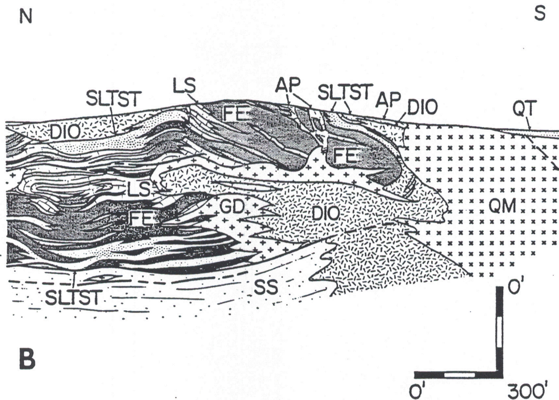
FIGURE 14. Geology along N-S cross section shown in figure 12. (A) shows the pre-magnetite geology; (B) shows the post-magnetite lithology and structures. Restored contacts are shown above the present ground surface. Ore containing more than 35 percent iron is shown by crosshatching.
