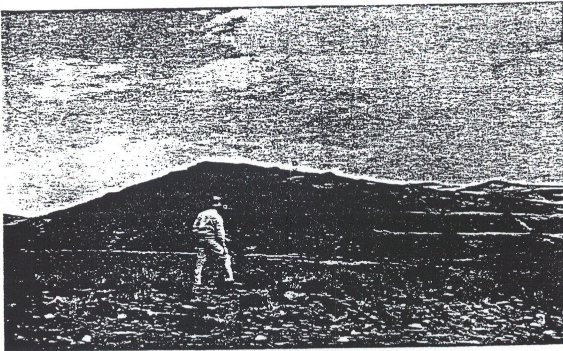
FIGURE 9. View looking east at the west flank of the hill where the southern third of the main orebody is exposed. The dark area extending down from the high point is high-grade hematite-magnetite. The east-west cross section (fig. 13) passes through the adit to the right of the man.
