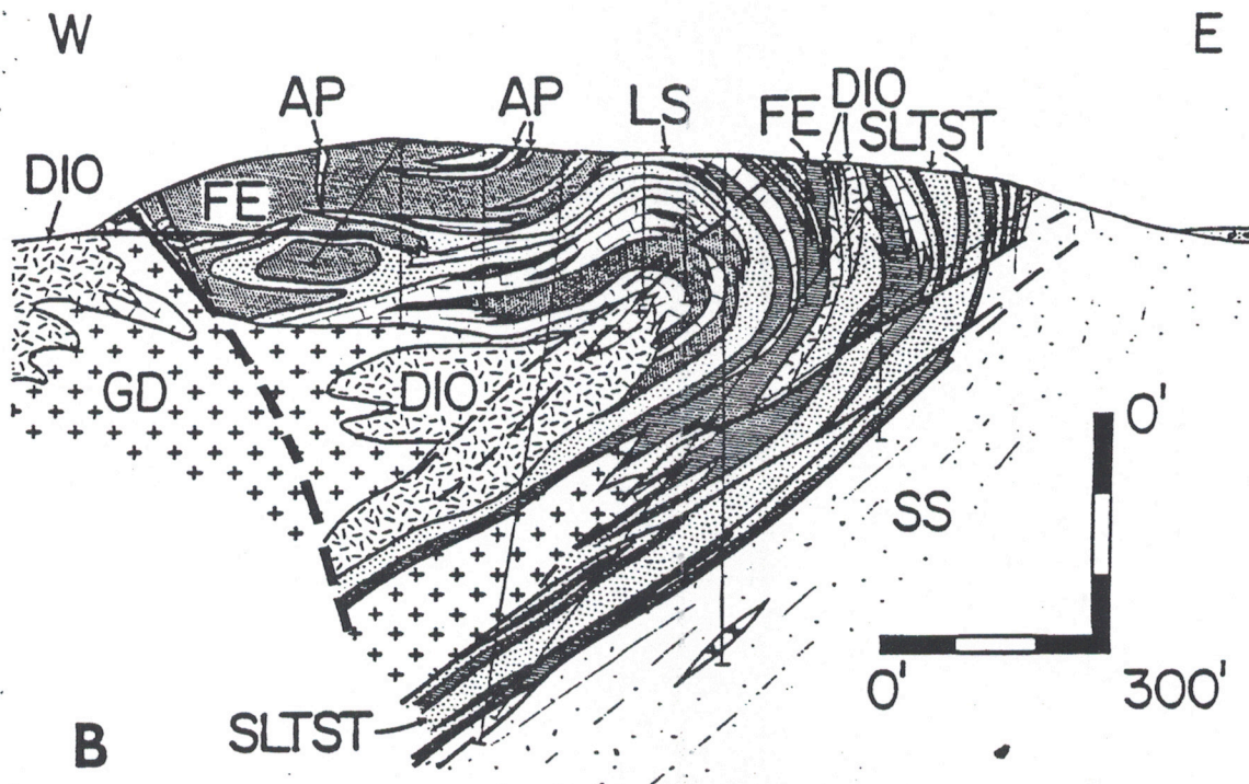
FIGURE 13. Geology along W-E cross section shown in figure 12. (A) shows the pre-magnetite geology; (B) shows the present lithology and structures. Areas of magnetite and magnetite/hematite ore containing more than 35 percent iron are crosshatched and labeled FE. Drill holes are shown as thin lines.
